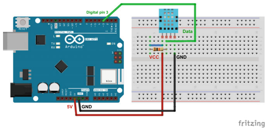
Fig. 4.4 Connecting DHT11 sensor to the Arduino
