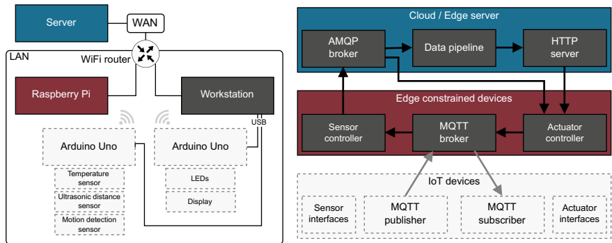
Fig. 9.1 Lab 6 setup
